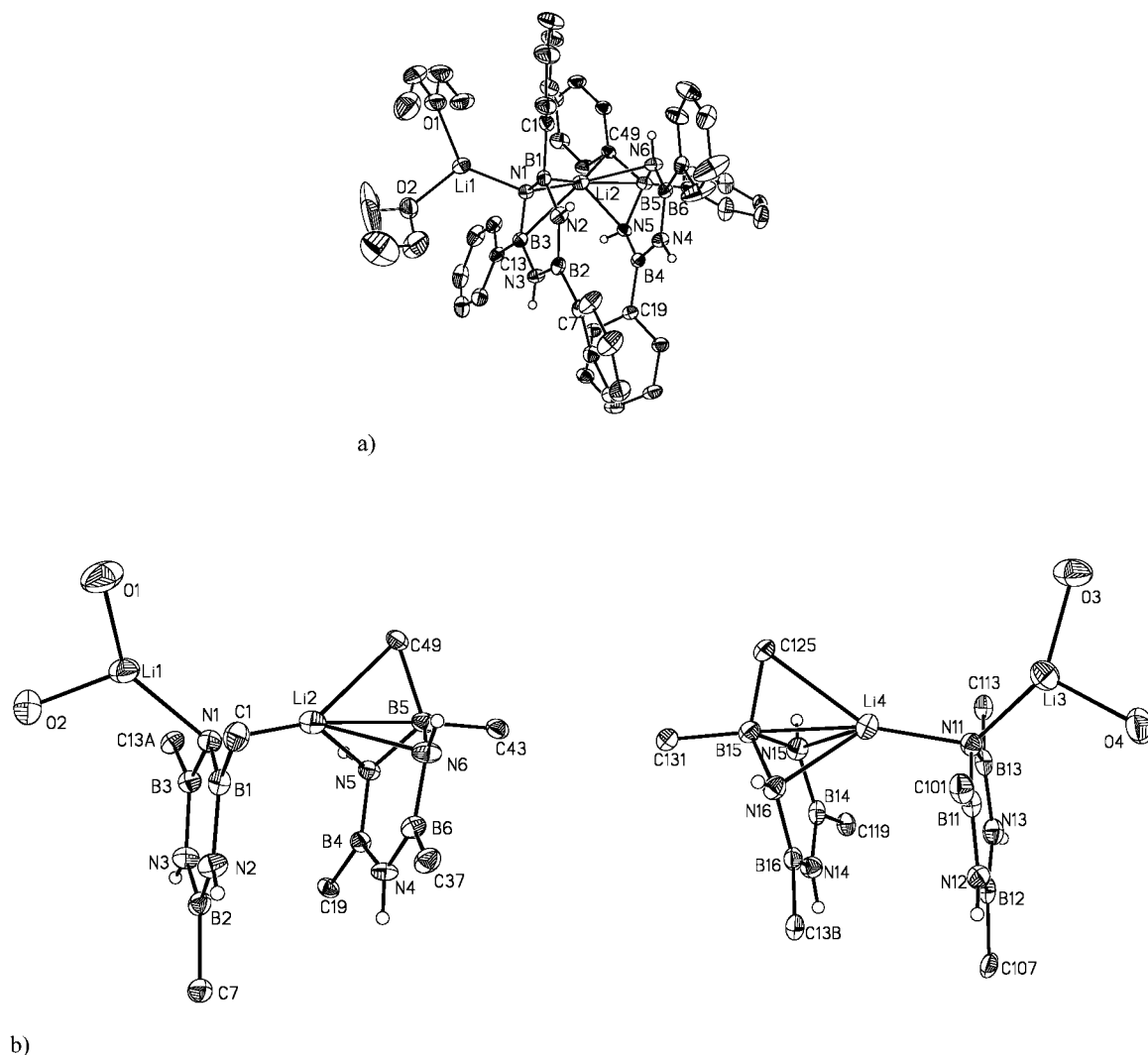
Figure 2. (a) Molecular structure of compound 7. Thermal ellipsoids are represented at a 25% probability scale. Selected bond lengths [Å] and angles [°]: O1–Li1 1.961(7), O2–Li1 1.968(9), N1–Li1 1.991(8), N1–Li2 2.025(8), N5–Li2 2.178(7), N6–Li2 2.213(8), B5–Li2 2.298(8), C49–Li2 2.416(7), O3–Li3 1.941(9), O4–Li3 1.950(9), N11–Li3 2.000(8), N11–Li4 2.012(7), N15–Li4 2.180(7), Li–N16 2.158(7), B1–C1 1.653(6), B1–C7 1.636(5), B2–C13 1.576(6), B3–C19 1.595(5), B4–C25 1.584(6), B5–C31 1.602(5), B6–C37 1.581(6), B7–C43 1.644(6), B7–C49 1.648(5), B8–C55 1.589(5), B9–C61 1.573(5), B10–C67 1.598(5), B11–C73 1.574(5), B12–C79 1.583(5), B1–C1 1.602(5), B2–C7 1.584(6), B3–C13 1.581(6), N4–C19 1.576(6), B5–C25 1.653(6), B5–C37 1.595(5), B5–C31 1.636(5), B6–C37 1.5895(5). O1–Li1–O2 104.6(4), O1–Li1–N1 111.9(4), O2–Li1–N1 137.1(4), N1–Li2–N5 131.3(4), N5–Li2–N6 67.3(2), N1–Li2–N6 136.1(3), Li1–N1–Li2 126(3), B1–N1–Li1 100.3(3), B1–N1–Li2 95.4(3), B3–N1–Li1 116.5(3), B1–N1–B3 117.0(3). Interplanar angles [°]: B1N2B3N3/B1N1B3 4.5, B1N2B3N3/N2B2N3 5.2, B1N2B3N3/C18C13C14 19.3, B1N2B3N3/C7C8C12 19.9, B1N2B3N3/C C16C 26.3; B4N5N6B6/B4N4B6 33.2, B4N5N6B6/N5B5N6 26.7, B4N5N6B6/C20C19C24 69.5, B4N5N6B6/ C38C37C42 16.7, N5B5N6/C44C43C48 90.5, N5B5N6/ C50C49C54 52.5. Second molecule: B11N12N13B13/B1111B13 2.7, B11N12N13B13/N12B23N13 4.7, B11N12N13B13/C102C101C106 150.2, B11N12N13B13/C108C107C112 14.8, B11N12N13B13/C114C113C118 6.9. (b) The core structure of the two independent molecules of 7.
