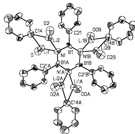
Figure 6. ORTEP plot of the molecular structure of compound 8 . Thermal ellipsoids represent a 25% probability. Selected bond lengths [Å] and angles [°]: Li1–O1 1.96(2), Li1–N1 2.03(2), Li1–C14 2.15(2), Li1···Li2 2.35(2), Li2–O2 1.92(2), Li2–N1 2.02(9), Li2–C14 2.22(2), Li2···B1 2.71(2), B1–N1 1.43(1), B1–N1B 1.46(1), B1–C14 1.63(2), B1···Li1B 2.60(2), N1–B1A 1.46(1), O1–Li1–N1 132(1), O1–Li1–C14 110.8(9), N1–Li1–C14 113.4(9), O2–Li2–N1 127.4(9), O2–Li2–C14 117(1), N1–Li2–C14 110.7(8), N1–B1–N1B 126(1), N1B–B1–C21 117(1), B1–N1–B1A 114(1), B1–N1–Li2 103(1), B1–N1–Li1 137.0(8), Li1–N1–Li2 71.0(7), B1A–N1–Li2 136.5(9), B1A–N1–Li1 95.2(9), Li1–C14–Li2 64.9(7). Interplanar angles [°]: B3N3/C1C2C6 39.9, B3N3/N1Li1Li2 53.8, N1Li1Li2/C14C15C19 90.0, C7Li1Li2/C14C15C19 90.0.
