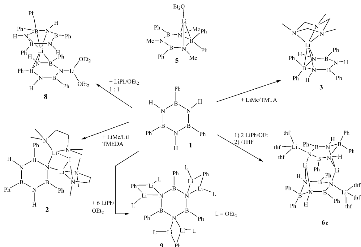
Scheme 1. Reactions of 1 with LiMe/LiI, LiMe and LiPh.
