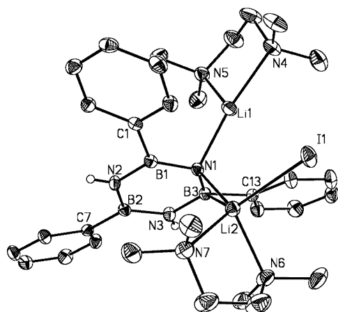
Figure 1. ORTEP plot of the molecular structure of 2 . Thermal ellipsoids are represented at a 25% probability scale. Selected bond lengths [Å] and angles [°]: B1–C1 1.595(4), B3–C13 1.598(4), B2–C7 1.582(4), Li1–N1 1.999(5), Li1–N4 2.148(5), Li1–N5 2.140(6), Li2–N1 2.094(5), Li2–N6 2.152(5), Li2–N7 2.223(5), Li2–I1 2.769(5), Li1...Li2 3.245(7), Li1–N1–Li2 104.9(2), B1–N1–Li1 107.3(2), B3–N1–Li1 111.6(2), B1–N1–Li2 109.5(2), B3–N1–Li2 105.3(2), N5–Li1–N4 85.3(2), N1–Li1–N5 108.2(2), N1–Li1–N4 166.5(3), N1–Li2–N6 126.2(2), N1–Li2–N7 116.3(2), N6–Li2–N7 84.2(2), B1–C1–C2 120.9(2), B2–C7–C8 121.7(2), C8–C7–C12 116.4(2), B3–C13–C14 122.6(2), C18–C13–C14 115.9(2). Torsion angles [°]: B2–N2–B1–C1 173.4, B2–N3–B3–C13 171.2, C8–C7–B2–N2 –20.7.
