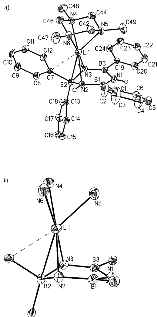
Figure 3. (a) ORTEP plot of the molecular structure of 3 . Thermal ellipsoids are represented at a 25% probability scale. Selected bond lengths [Å] and angles [°]: Li1–N2 2.186(7), Li1–N3 2.235(7), Li1–N4 2.165(7), Li1–N5 2.188(7), Li1–N6 2.196(7), Li1–C7 2.453(7), B1–C1 1.580(5), B2–C7 1.650(5), B2–C13 1.630(6), B3–C19 1.585(6), N2–Li1–N4 172.5(3), N2–Li1–N5 118.3(3), N2–Li1–N6 109.5(3), N3–Li1–N4 117.1(3), N3–Li1–N5 117.0(3), N3–Li1–N6 120.6(3), N3–Li1–N6 174.9(4), N4–Li1–N5 65.1(2), N4–Li1–N6 65.1(2), N5–Li1–N6 64.5(2), N1–B1–C13 119.8(3), N2–B1–C1 122.9(3), N2–B2–C7 109.6(3), N2–B2–C13 112.0(3), C7–B2–C13 107.2(3), N3–B3–C19 121.8(3), B1–N2–Li1 98.1(3), B2–N3–Li1 72.5(2), B2–N2–Li1 74.2(3), B3–N3–Li1 99.6(3). Torsion angles [°]: N1–B1–N2–B2 11.2, B1–N2–B2–N3 –32.4, N2–B2–N3–B3 35.2, B2–N3–B3–N1 –17.7, N3–B3–N1–B1 –10.6, B3–N1–B1–N2 13.8. Interplanar angles [°]: B1N2B3N3/B1N1B3 10.9, B1N2B3N3/N2B2N3 27.4, B1N2B3N3/C6C1C2 22.1, B1N2B3N3/C8C7C12 68.8, B1N2B3N3/C14C13C18 77.1, B1N2B3N3/C20C19C24 23.6. (b) Core structure of compound 3 showing the geometry around the Li1 atom.
