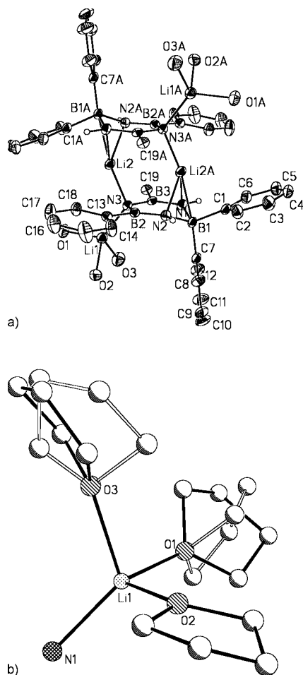
Figure 5. (a) Molecular structure of compound 6c . Thermal ellipsoids are depicted on a 25% probability scale. Only the ipso -C atoms of the phenyl groups are shown for clarity. Selected bond lengths [Å] and angles [°]: Li1–O1 1.977(6), Li1–O2 2.024(6), Li1–O3 2.084(6), Li1–N1 2.073(6), Li2–N1 2.003(6), Li2–N2A 2.137(6), Li2–N3A 2.169(6), Li2···Li2A 3.29(1), Li2A–B1 2.641(6), Li2–B1A 2.311(6), B1–C1 1.601(4), B2–C7 1.635(5), B2–C13 1.652(5), B3–C19 1.603(4), O1–Li1–O2 103.9(3), O1–Li1–O3 95.9(2), O2–Li1–O3 95.3(3), N1–Li1–O1 124.1(3), N1–Li1–O2 113.1(3), N1–Li1–O3 119.7(3), N1–Li2–N2A 132.5(3), N1–Li2–N3A 135.0(3), N2A–Li2–N3A 68.3(2), Li1–N1–Li2 118.3(2), B1–N1–Li1 111.2(2), B3–N1–Li1 107.0(2), B1–N1–Li2 101.5(2), B3–N1–Li2 103.0(2). Interplanar angles [°]: B1N1N3B3/B1N1B3 2.6, B1N1N3B3/N2B2N3 27.8, B1N1N3B3/C19C20C24 12.9, B1N1N3B3/C2C1C6 7.6, N2B2N3/C14C13C18 50.5, N2B2N3/C8C7C12 125, C13C14C18/C8C7C12 75.5. (b) Plot of the disordered THF molecules in compound 6c .
