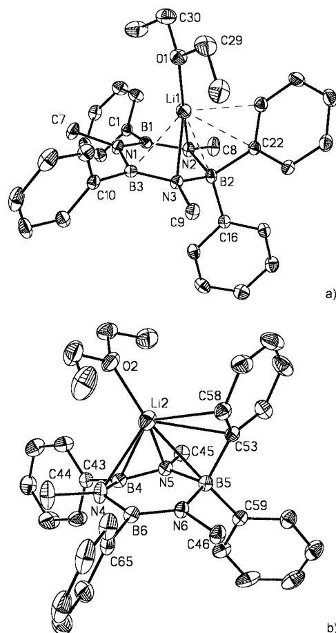
Figure 4. (a) ORTEP plot of one of the two isomeric molecules of compound 5a . Thermal ellipsoids are represented at a 25% probability scale. Selected bond lengths [Å] and angles [°]: Li1–O1 1.928(4), Li1–N1 2.167(5), Li1–N2 2.349(4), Li1–N3 2.518(5), Li1–B2 2.652(5), Li1–B3 2.420(5), Li1–C4 2.454(5), Li1–O1 1.928(5), B1–C1 1.587(4), B2–C16 1.632(4), B2–C22 1.665(3), B3–C10 1.584(3), O1–Li1–N1 120.5(2), O1–Li1–N2 157.4(3), O1–Li1–N3 134.2(3), N1–Li1–N2 60.6(1), N1–Li1–N3 62.8(1), N2–Li1–N3 67.9(1). Interplanar angles [°]: B1N2N3B3/B1N1B3 14.0, B1N2N3B3/N2B2N3 10.8, B1N2N3B3/C1C2C6 120.0, B1N2N3B3/C10C11C15 107.4, B1N2N3B3/C16C17C21 91.5, B1N2N3B3/C22C23C27 117.4. (b) The structure of the second isomer of compound 5b . Selected bond lengths [Å] and angles [°]: Li2–N4 2.143(6), Li2–N5 2.426(3), Li2–B4 2.485(6), Li2–B5 2.400(5), Li2–C53 2.414(6), Li2–C58 2.399(6), B4–C43 1.587(4), B5–C53 1.662(4), B5–C59 1.628(4), B6–C65 1.569(4), O2–Li2–N4 114.6(2), O2–Li2–N5 136.5(3), N4–Li2–N5 64.4(2), N4–B4–Li2 73.4(2), N5–B4–Li2 62.2(2), B4–N4–Li2 71.5(2), B4–N5–Li2 82.2(2). Interplanar angles [°]: B4N4N6B6/B4N4B6 10.7, B4N5N6B6/N5B5N6 2.8.
